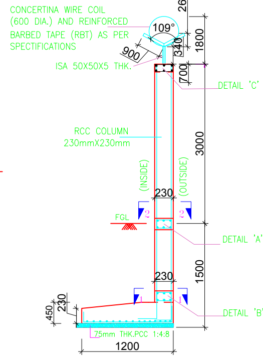
SECTION Y-Y
