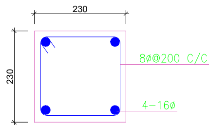
VIEW 2-2 (R.C.C COLUMN)
