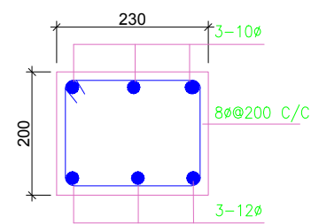
DETAIL 'B'
