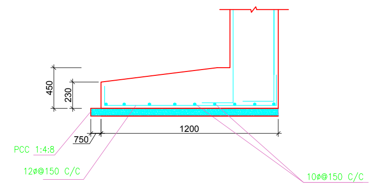
DETAIL OF FOOTING
