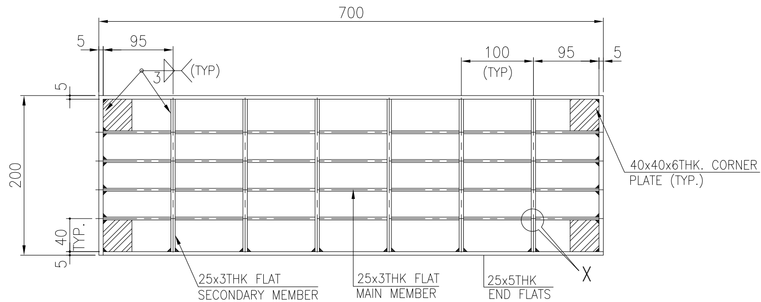
DETAILS OF 700x200 GRATING
